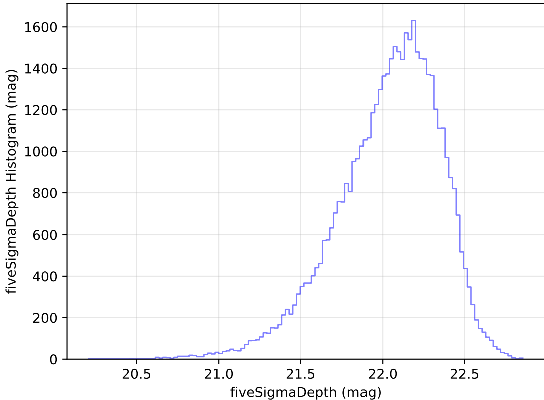
internal_u_expt30_nscale0.9v3.4_10yrs Yr 1 y band: fiveSigmaDepth Histogram
