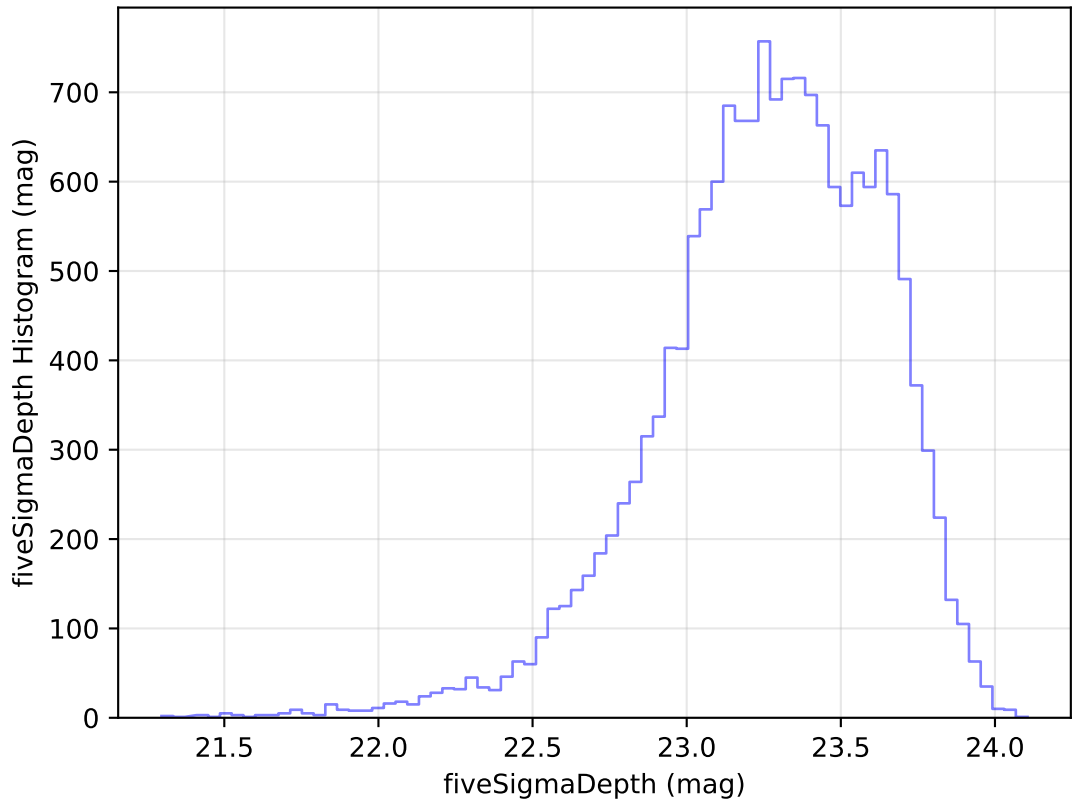
internal_u_expt30_nscale0.9v3.4_10yrs Yr 1 u band: fiveSigmaDepth Histogram
