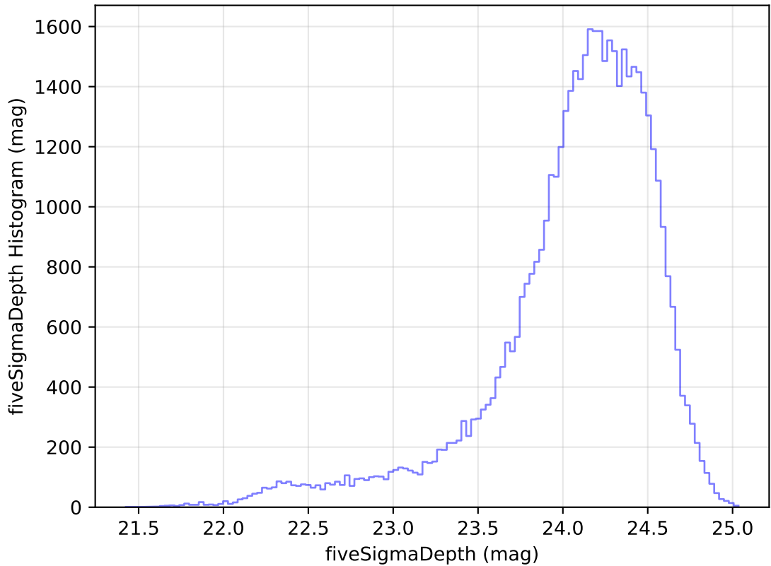
internal_u_expt30_nscale0.9v3.4_10yrs Yr 1 r band: fiveSigmaDepth Histogram
