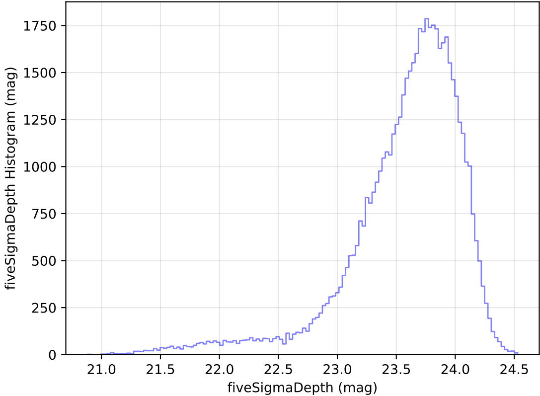
internal_u_expt30_nscale0.9v3.4_10yrs Yr 1 i band: fiveSigmaDepth Histogram
