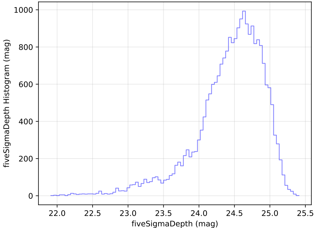
internal_u_expt30_nscale0.9v3.4_10yrs Yr 1 g band: fiveSigmaDepth Histogram
