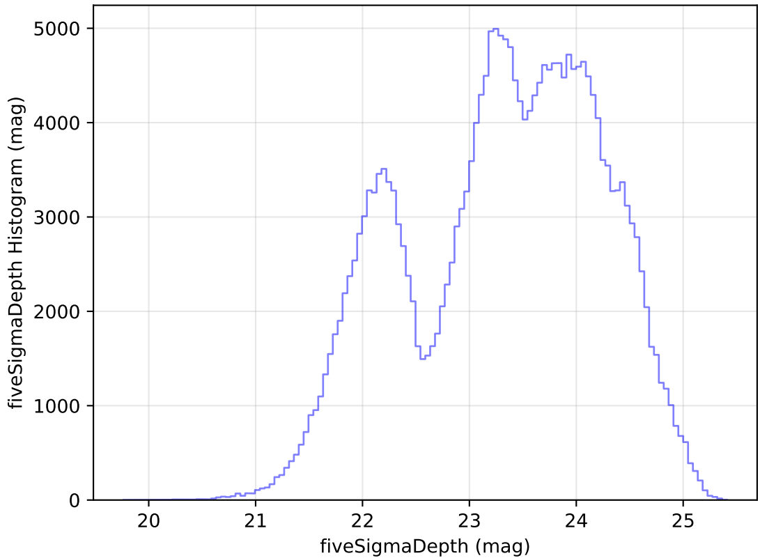
internal_u_expt30_nscale0.9v3.4_10yrs Yr 1 all bands: fiveSigmaDepth Histogram
