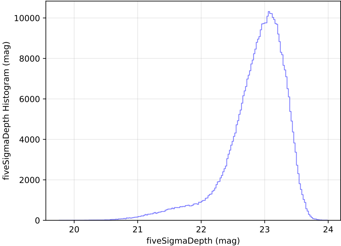
internal_u_expt30_nscale0.9v3.4_10yrs WFD z band: fiveSigmaDepth Histogram
