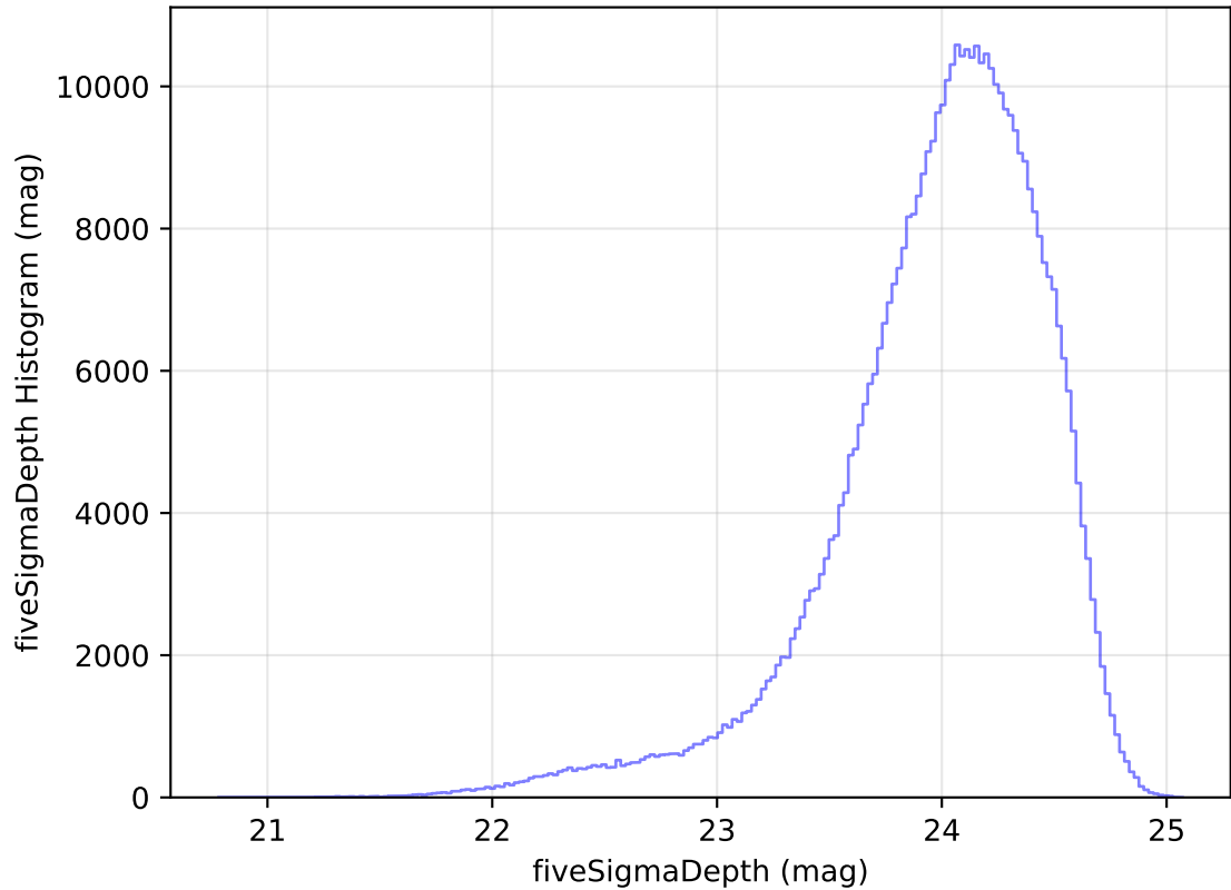
internal_u_expt30_nscale0.9v3.4_10yrs WFD r band: fiveSigmaDepth Histogram
