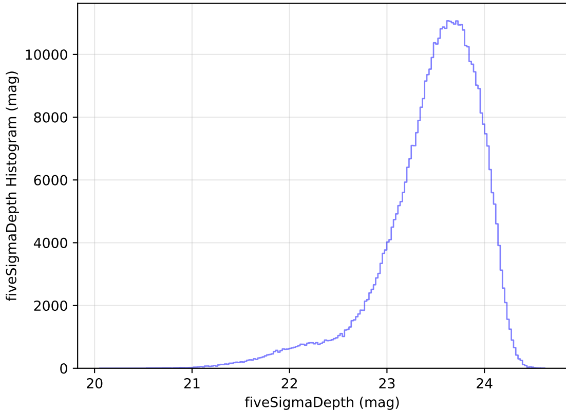
internal_u_expt30_nscale0.9v3.4_10yrs WFD i band: fiveSigmaDepth Histogram
