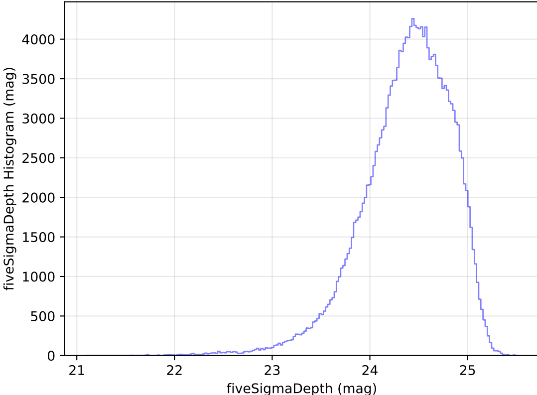
internal_u_expt30_nscale0.9v3.4_10yrs WFD g band: fiveSigmaDepth Histogram
