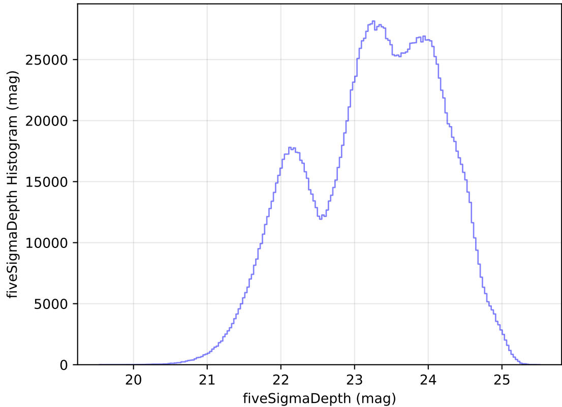
internal_u_expt30_nscale0.9v3.4_10yrs WFD all bands: fiveSigmaDepth Histogram
