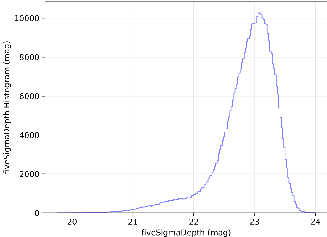
internal_u_expt30_nscale0.9v3.4_10yrs All sky z band: fiveSigmaDepth Histogram
