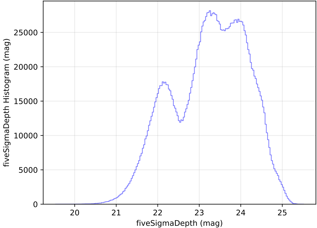
internal_u_expt30_nscale0.9v3.4_10yrs All sky all bands: fiveSigmaDepth Histogram
