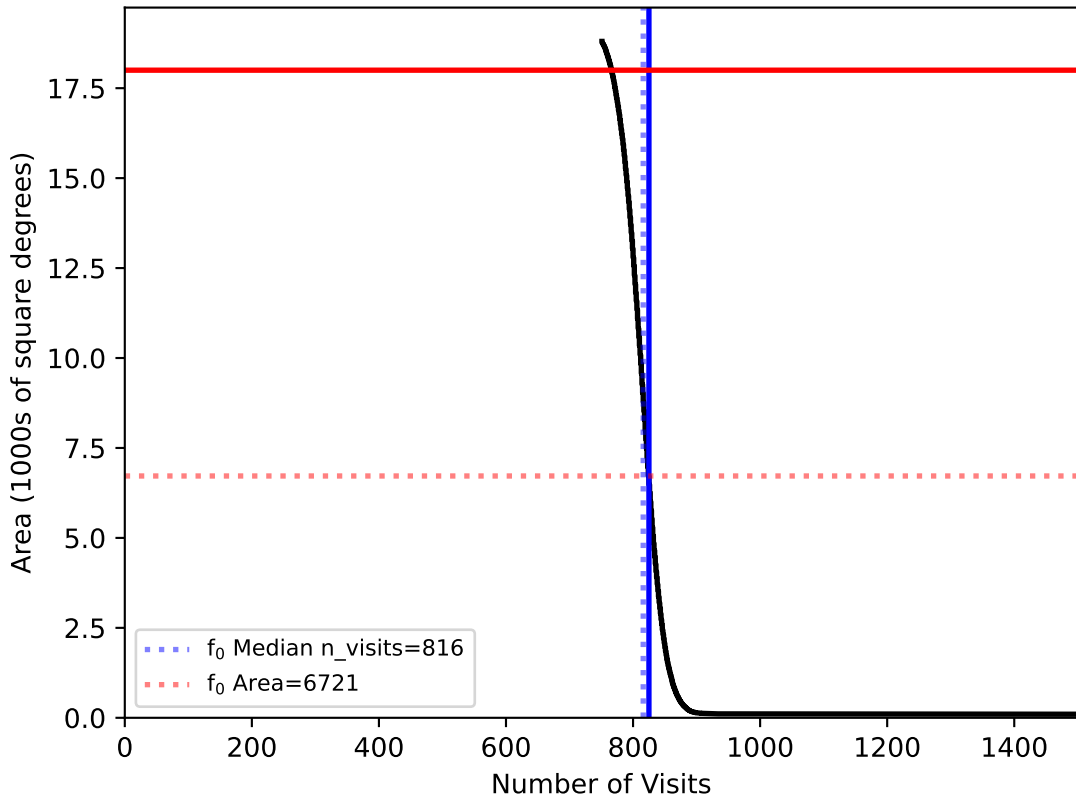
internal_u_expt30_nscale0.9v3.4_10yrs WFD: fO
