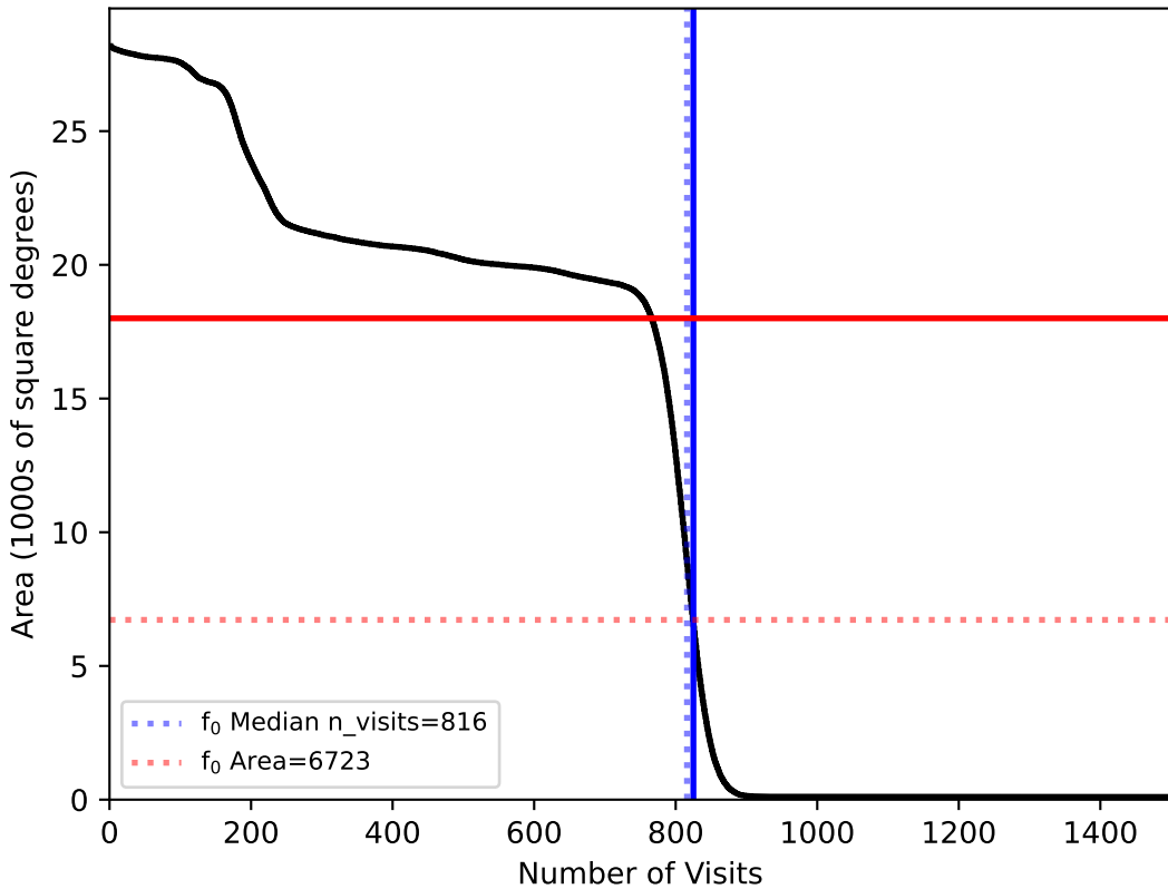
internal_u_expt30_nscale0.9v3.4_10yrs All sky: f0
