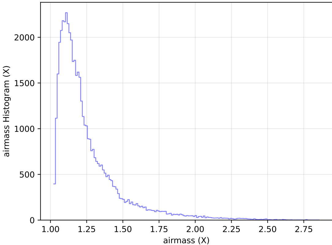
internal_u_expt30_nscale0.9v3.4_10yrs Yr 1 y band: airmass Histogram
