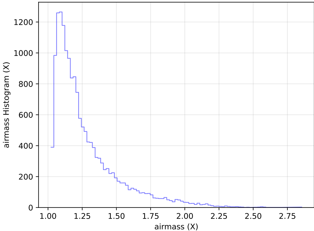
internal_u_expt30_nscale0.9v3.4_10yrs Yr 1 u band: airmass Histogram
