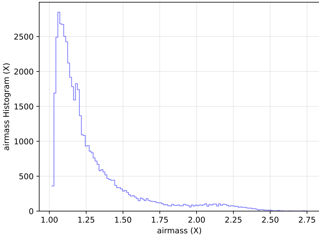
internal_u_expt30_nscale0.9v3.4_10yrs Yr 1 r band: airmass Histogram
