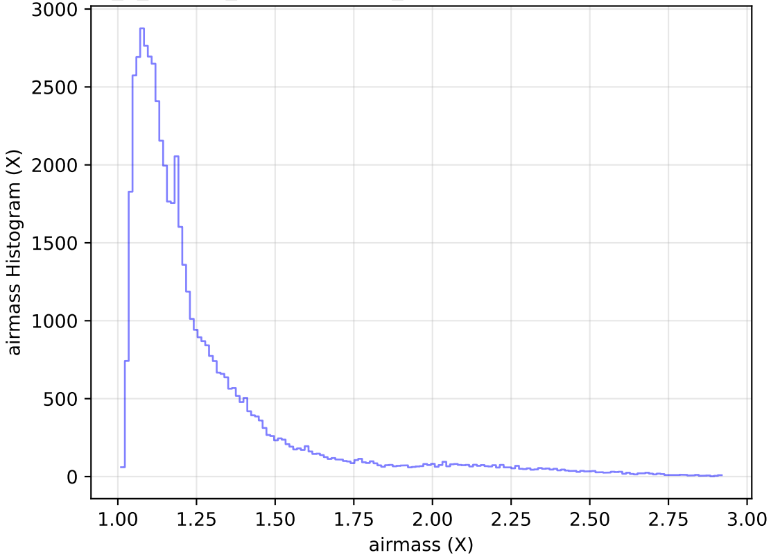
internal_u_expt30_nscale0.9v3.4_10yrs Yr 1 i band: airmass Histogram
