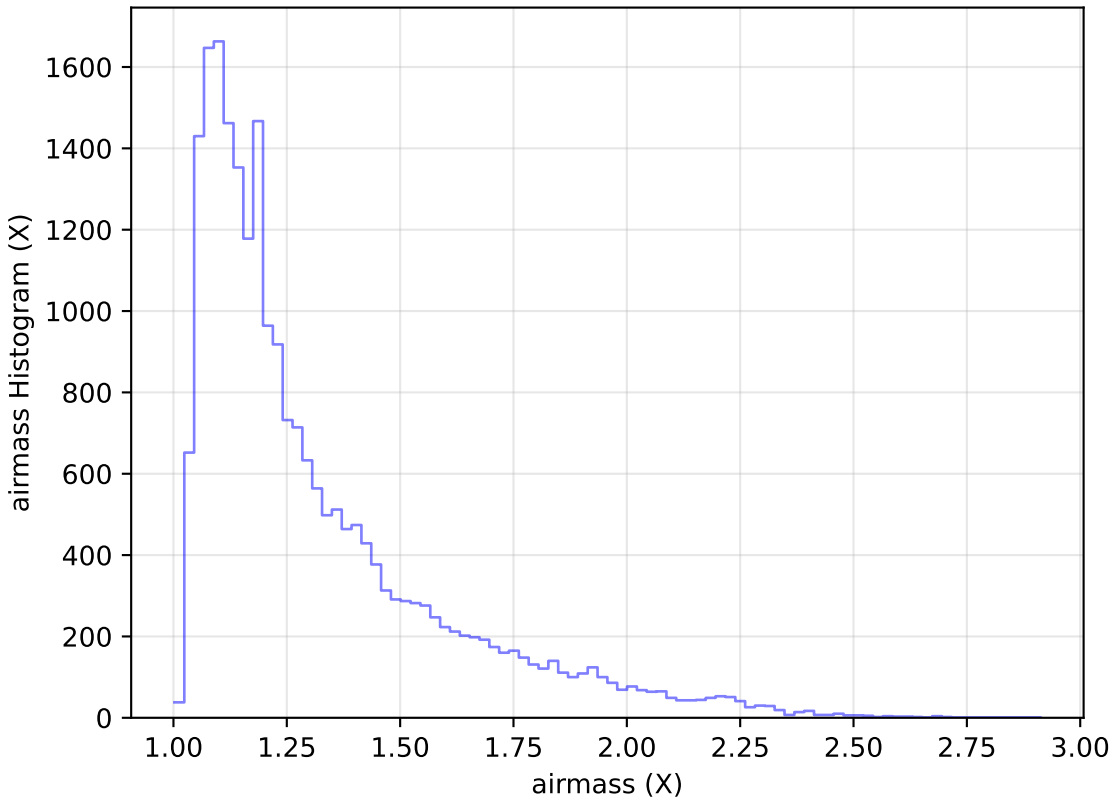
internal_u_expt30_nscale0.9v3.4_10yrs Yr 1 g band: airmass Histogram
