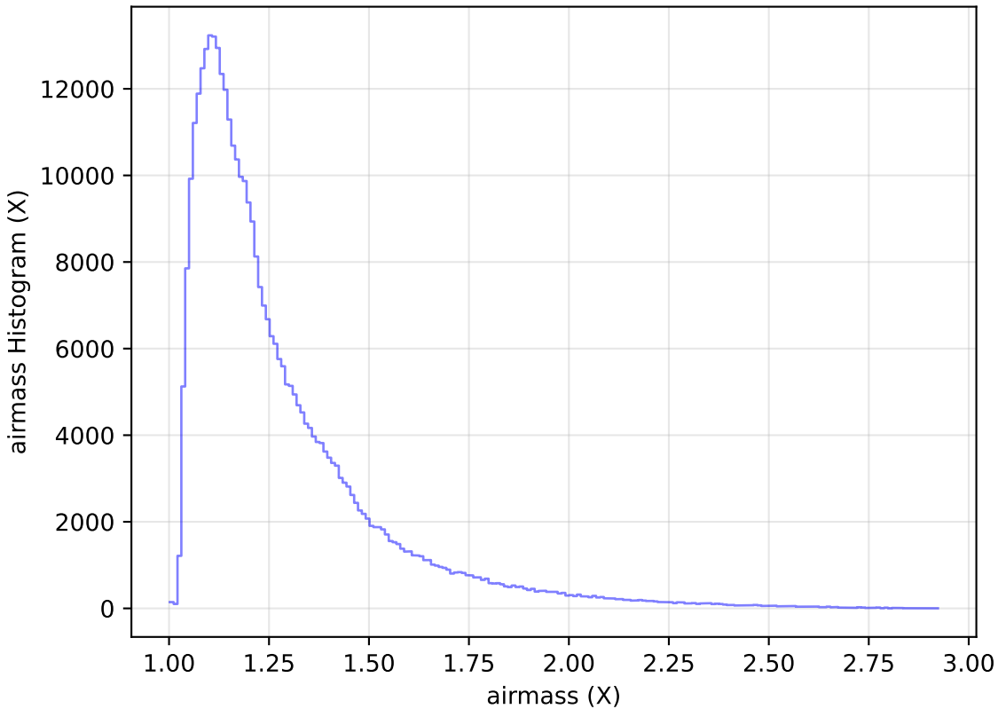
internal_u_expt30_nscale0.9v3.4_10yrs WFD y band: airmass Histogram
