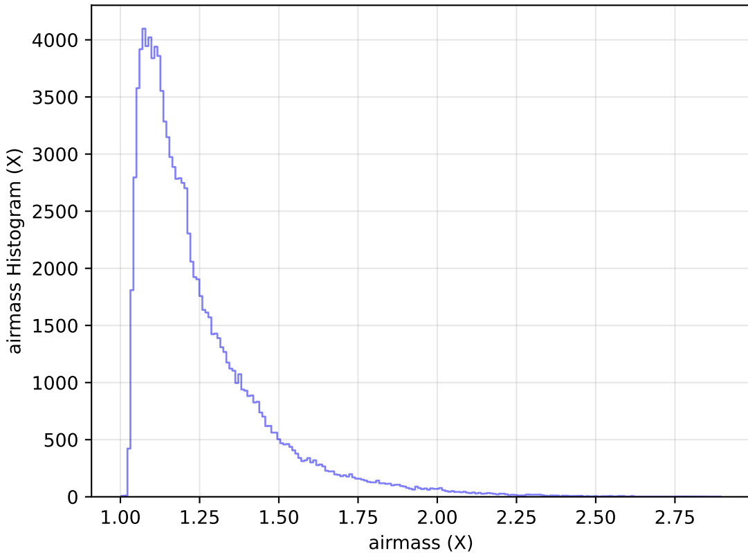
internal_u_expt30_nscale0.9v3.4_10yrs WFD u band: airmass Histogram
