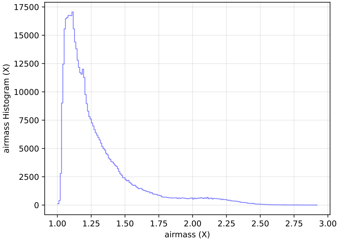
internal_u_expt30_nscale0.9v3.4_10yrs WFD r band: airmass Histogram
