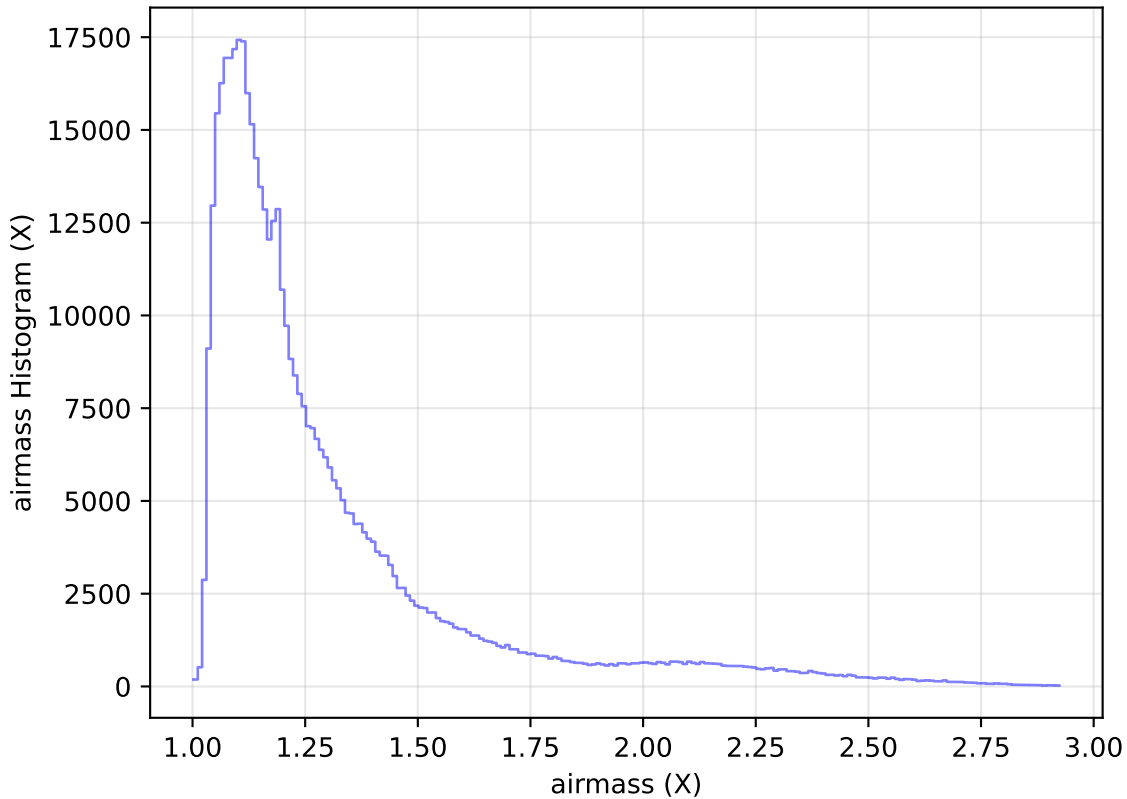
internal_u_expt30_nscale0.9v3.4_10yrs WFD i band: airmass Histogram
