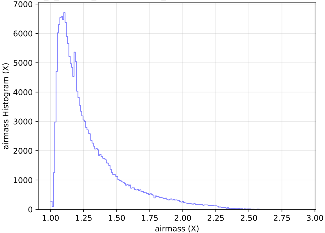
internal_u_expt30_nscale0.9v3.4_10yrs WFD g band: airmass Histogram
