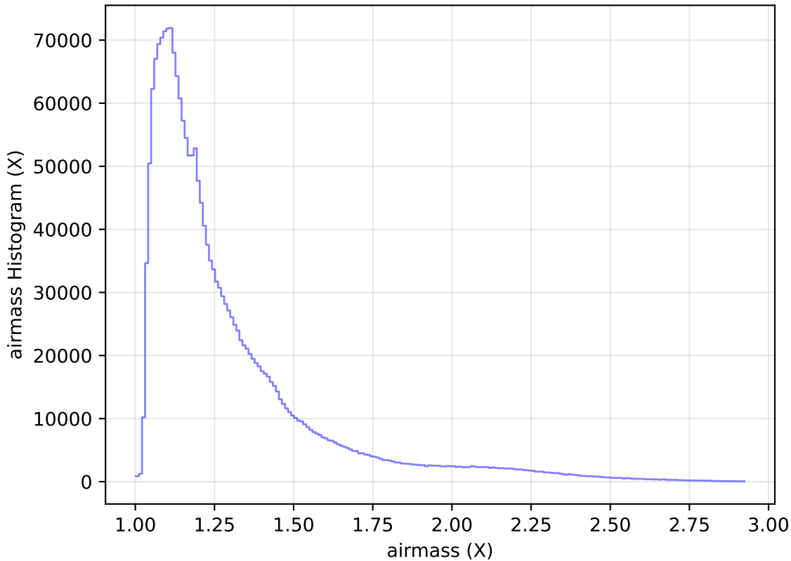
internal_u_expt30_nscale0.9v3.4_10yrs WFD all bands: airmass Histogram
