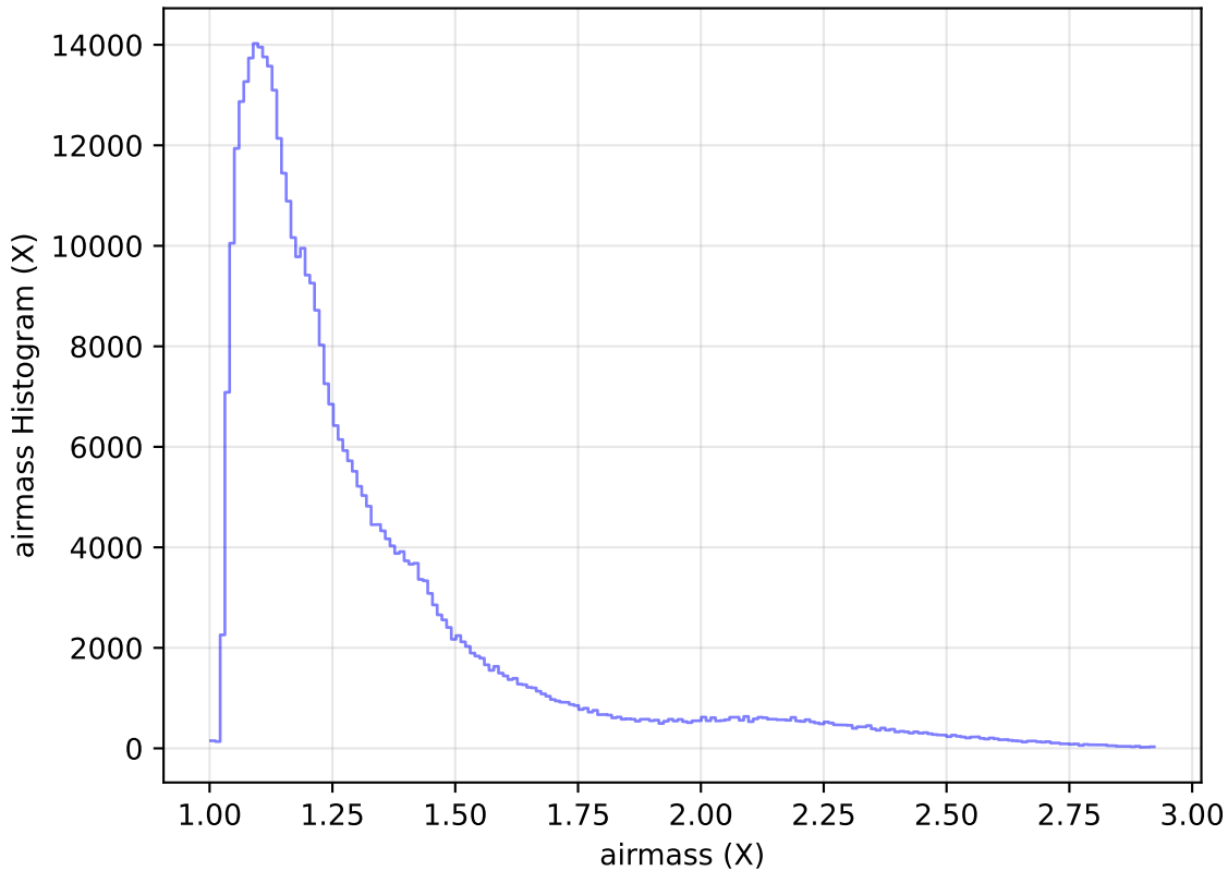
internal_u_expt30_nscale0.9v3.4_10yrs All sky z band: airmass Histogram
