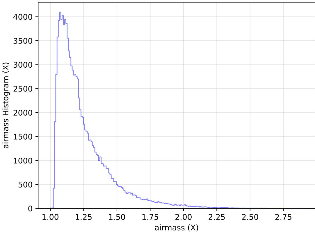
internal_u_expt30_nscale0.9v3.4_10yrs All sky u band: airmass Histogram
