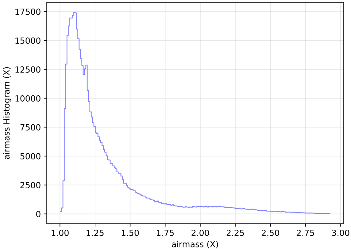
internal_u_expt30_nscale0.9v3.4_10yrs All sky i band: airmass Histogram
