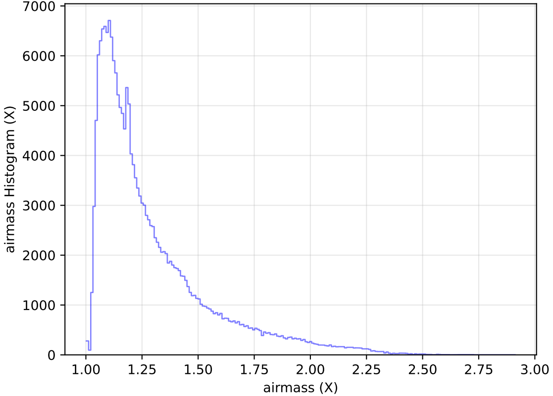
internal_u_expt30_nscale0.9v3.4_10yrs All sky g band: airmass Histogram
