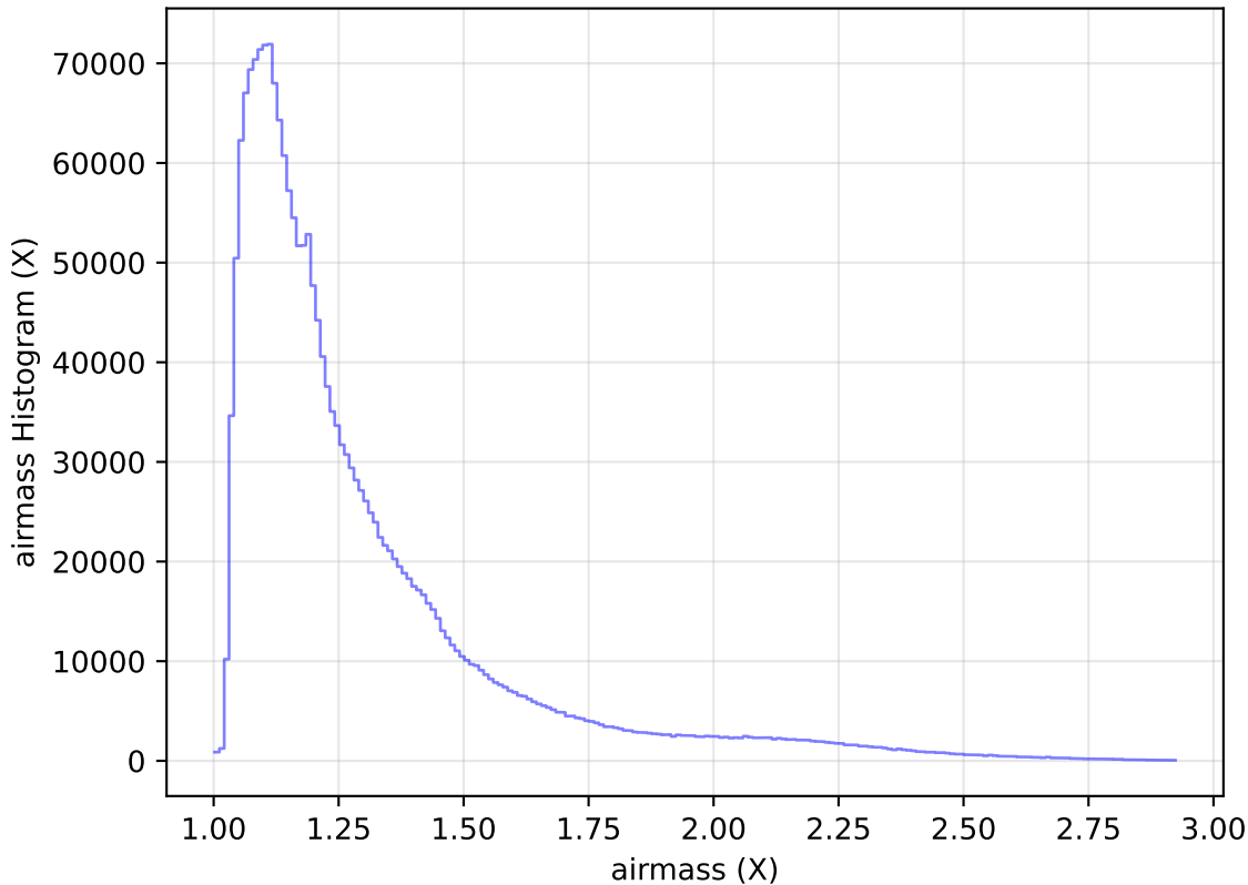
internal_u_expt30_nscale0.9v3.4_10yrs All sky all bands: airmass Histogram
