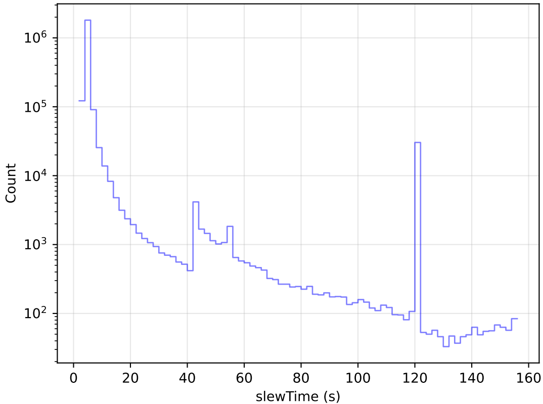
internal_u_expt30_nscale0.9v3.4_10yrs All visits: Slew Time Histogram
