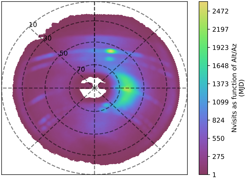
internal_u_expt30_nscale0.9v3.4_10yrs z band: Nvisits as function of Alt/Az
