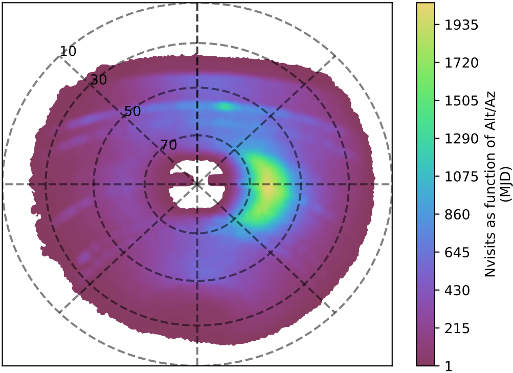
internal_u_expt30_nscale0.9v3.4_10yrs y band: Nvisits as function of Alt/Az
