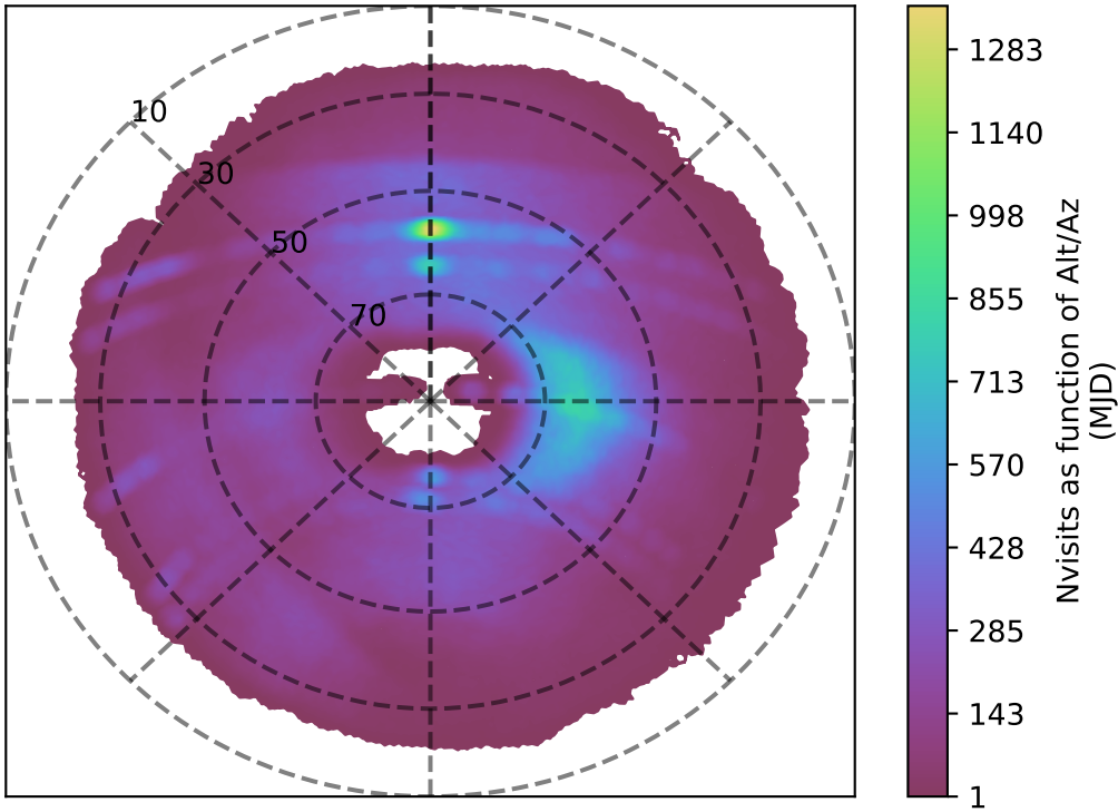
internal_u_expt30_nscale0.9v3.4_10yrs g band: Nvisits as function of Alt/Az
