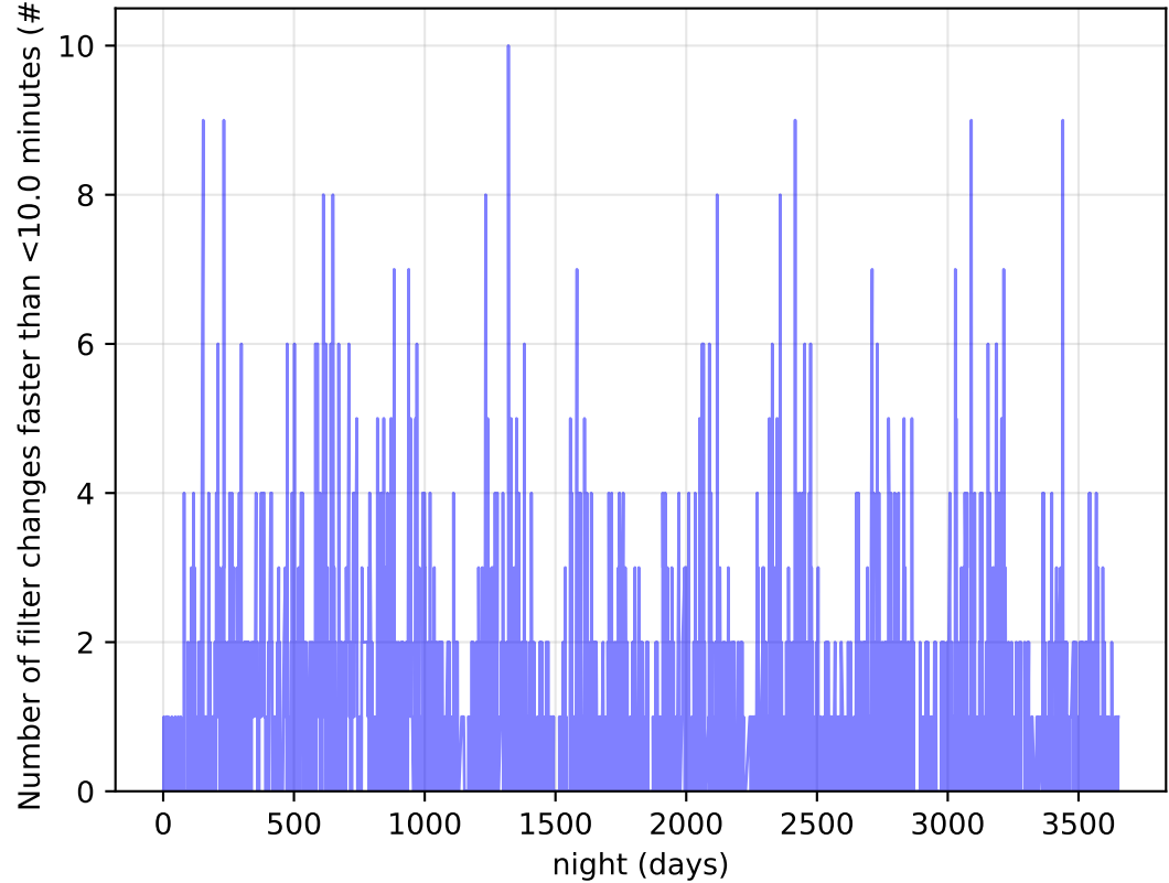
internal_u_expt30_nscale0.9v3.4_10yrs Per Night: Number of filter changes faster than <10.0 minutes
