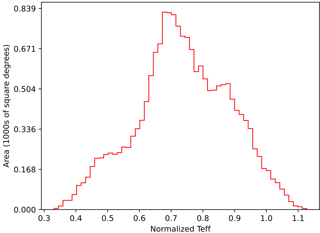
internal_u_expt30_nscale0.9v3.4_10yrs WFD i band: Normalized Teff
