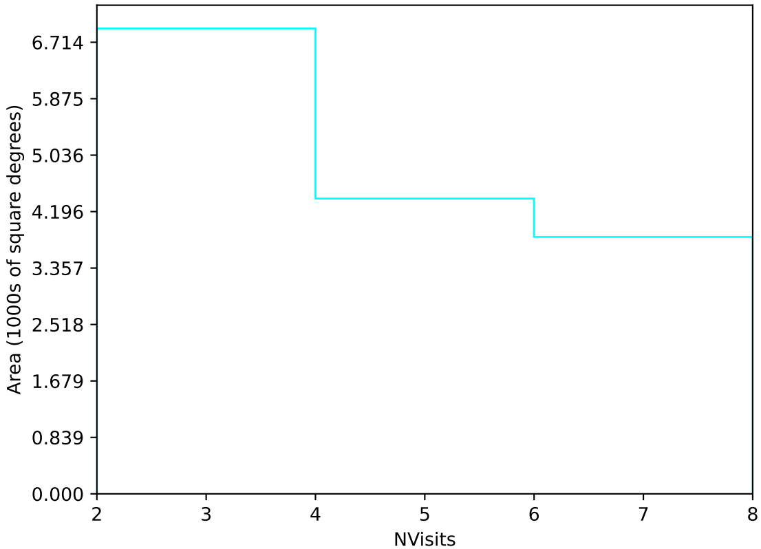
internal_u_expt30_nscale0.9v3.4_10yrs Yr 3-4 u band: NVisits
