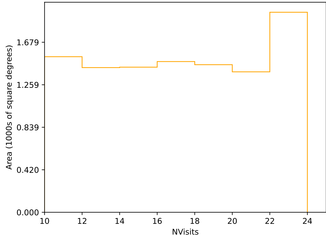
internal_u_expt30_nscale0.9v3.4_10yrs Yr 3-4 r band: NVisits
