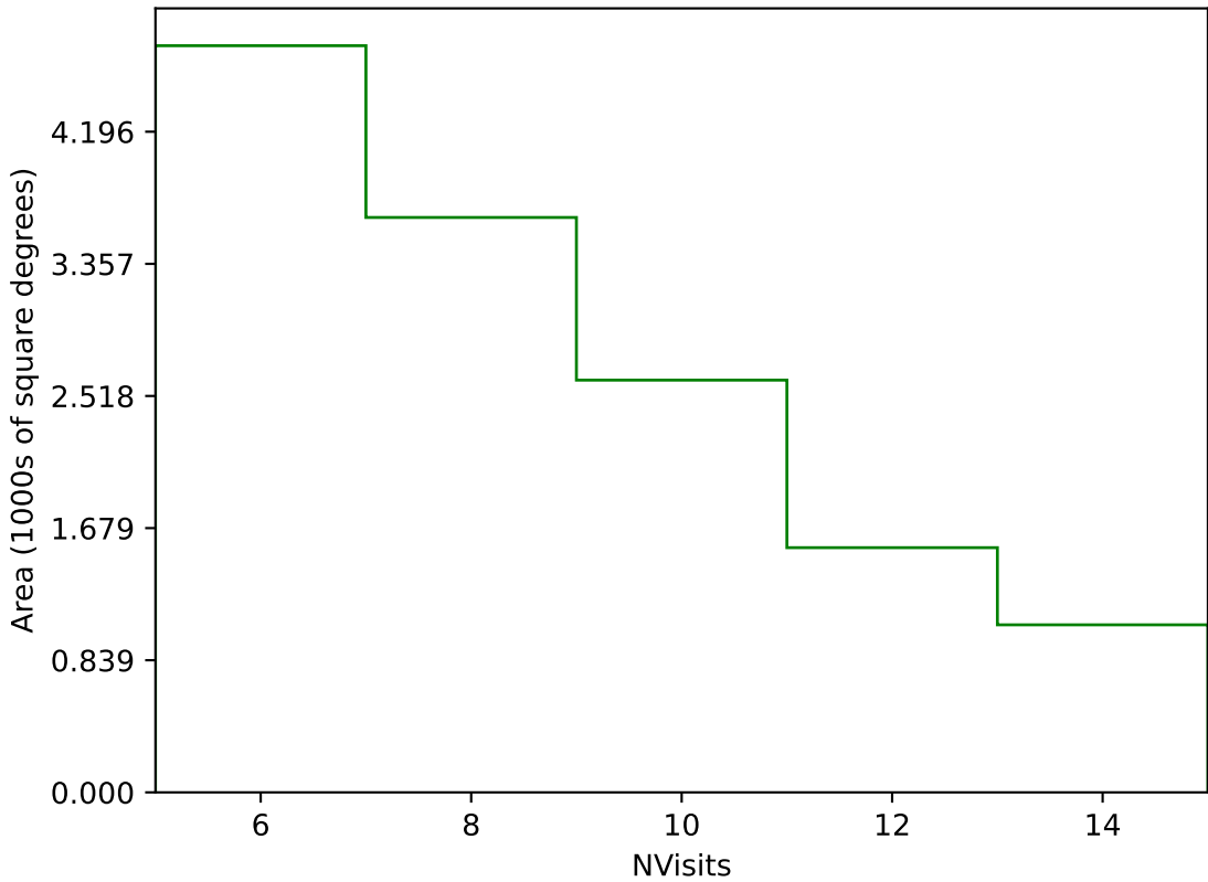
internal_u_expt30_nscale0.9v3.4_10yrs Yr 3-4 g band: NVisits
