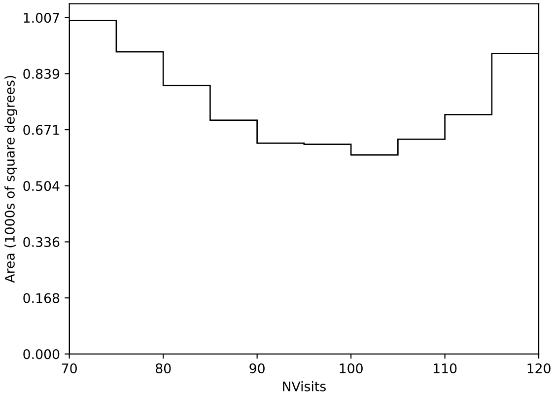
internal_u_expt30_nscale0.9v3.4_10yrs Yr 3-4 all bands: NVisits
