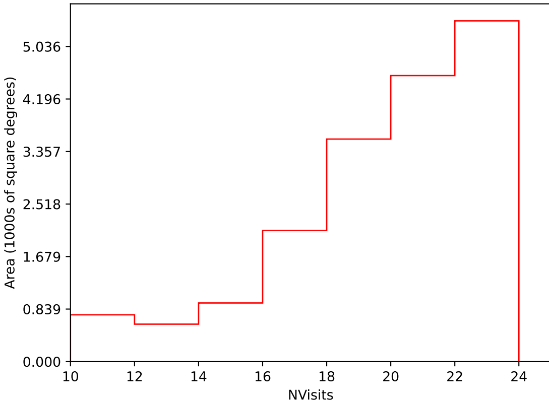
internal_u_expt30_nscale0.9v3.4_10yrs Yr 1 i band: NVisits
