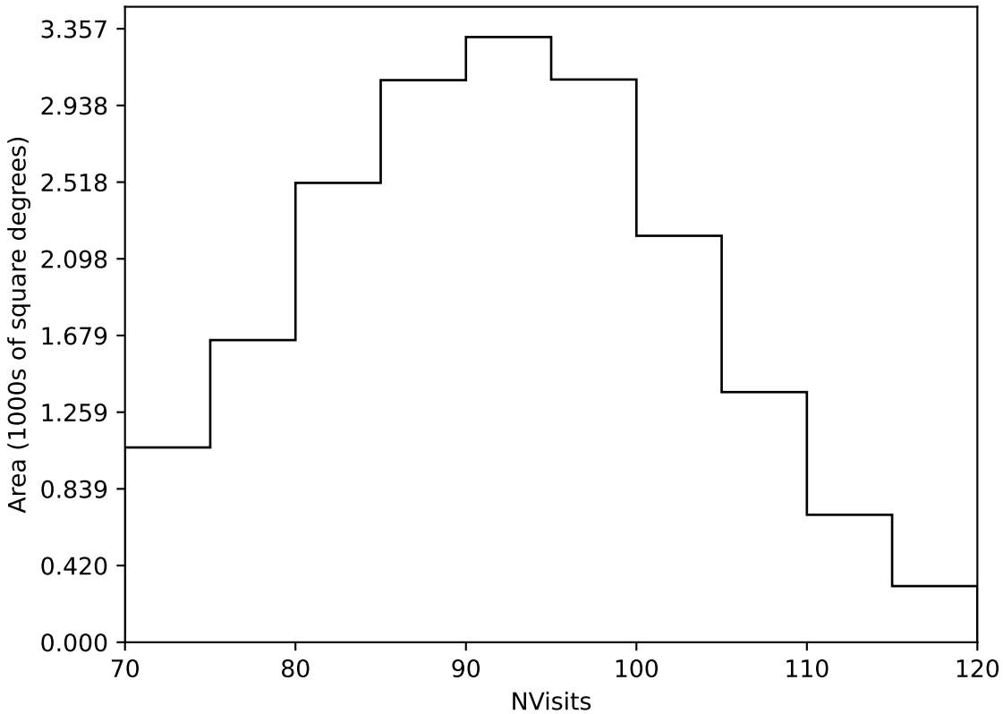
internal_u_expt30_nscale0.9v3.4_10yrs Yr 1 all bands: NVisits
