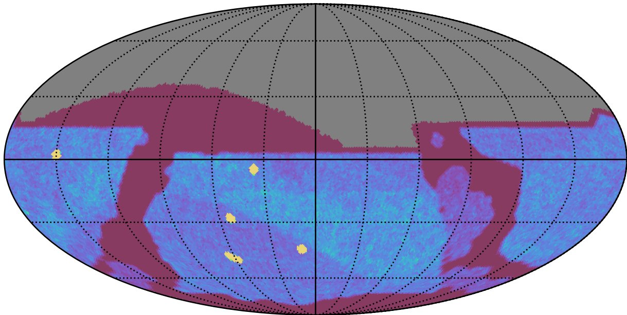
internal_u_expt30_nscale0.9v3.4_10yrs All sky z band: NVisits
