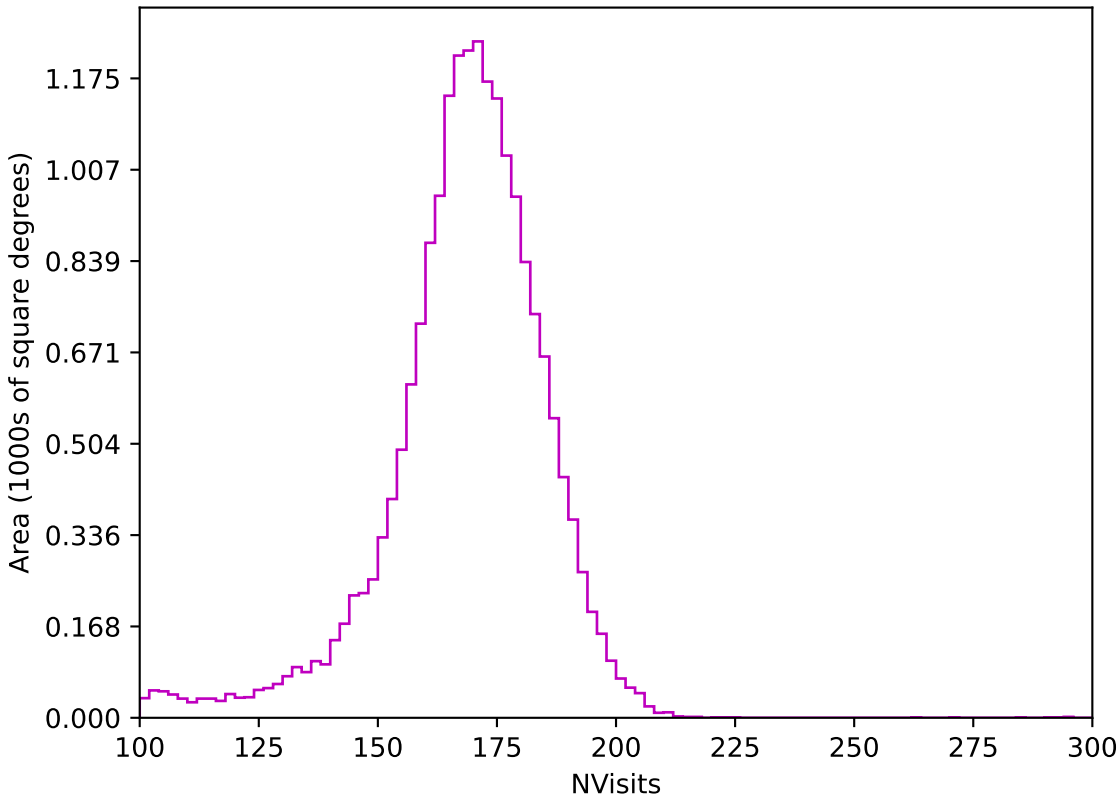
internal_u_expt30_nscale0.9v3.4_10yrs All sky z band: NVisits
