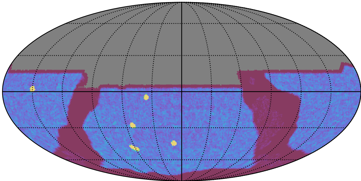
internal_u_expt30_nscale0.9v3.4_10yrs All sky y band: NVisits
