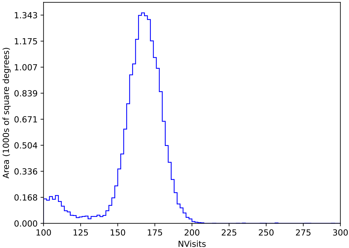
internal_u_expt30_nscale0.9v3.4_10yrs All sky y band: NVisits
