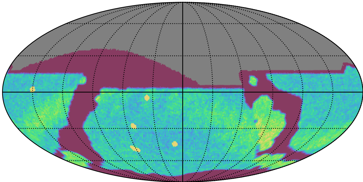
internal_u_expt30_nscale0.9v3.4_10yrs All sky r band: NVisits
