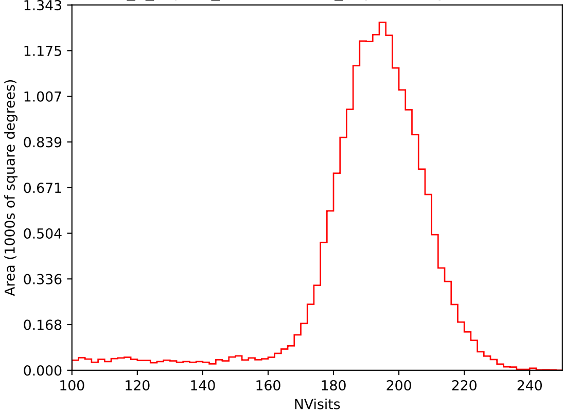
internal_u_expt30_nscale0.9v3.4_10yrs All sky i band: NVisits
