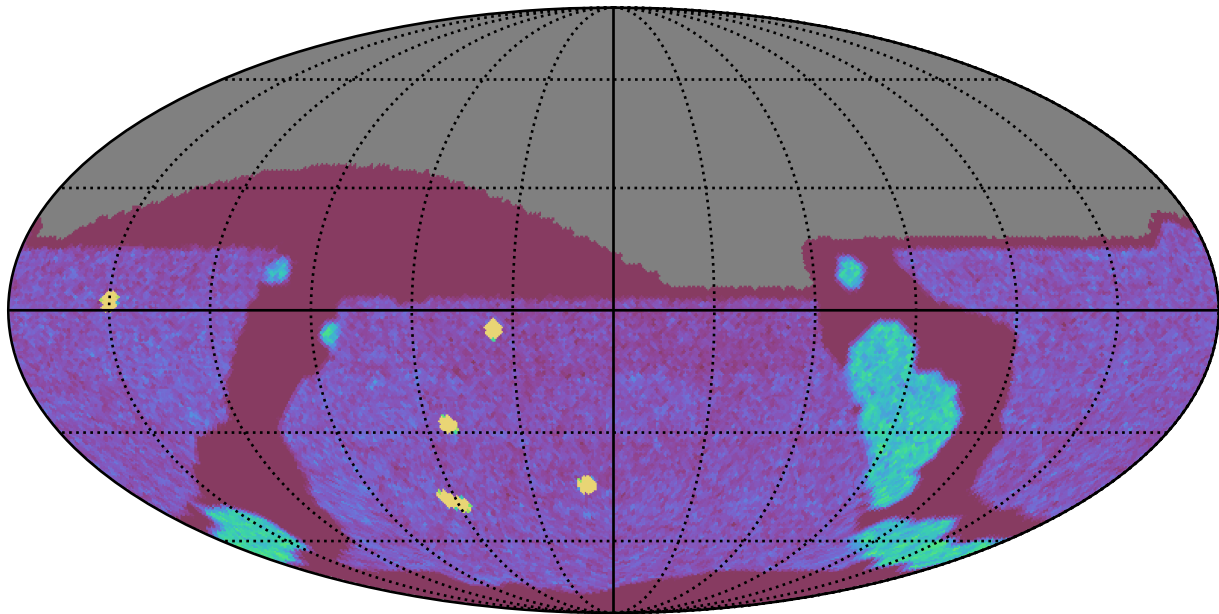
internal_u_expt30_nscale0.9v3.4_10yrs All sky g band: NVisits
